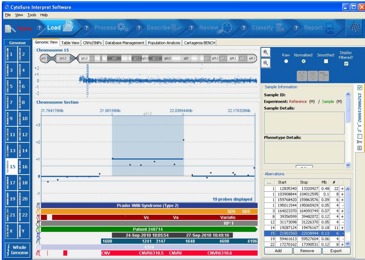
Figure 2: Reliable detection of small aberrations. DNA labelled using the CytoSure Genomic DNA Labelling Kit was run on a CytoSure ISCA 8 x 60K array. CytoSure Interpret Software combined with high DNA signal intensity allowed detection of a small (130 kb) DNA amplification.
